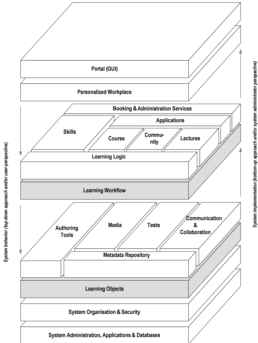
Figure 2: LMS-architecture [Milius 2002, 166]
