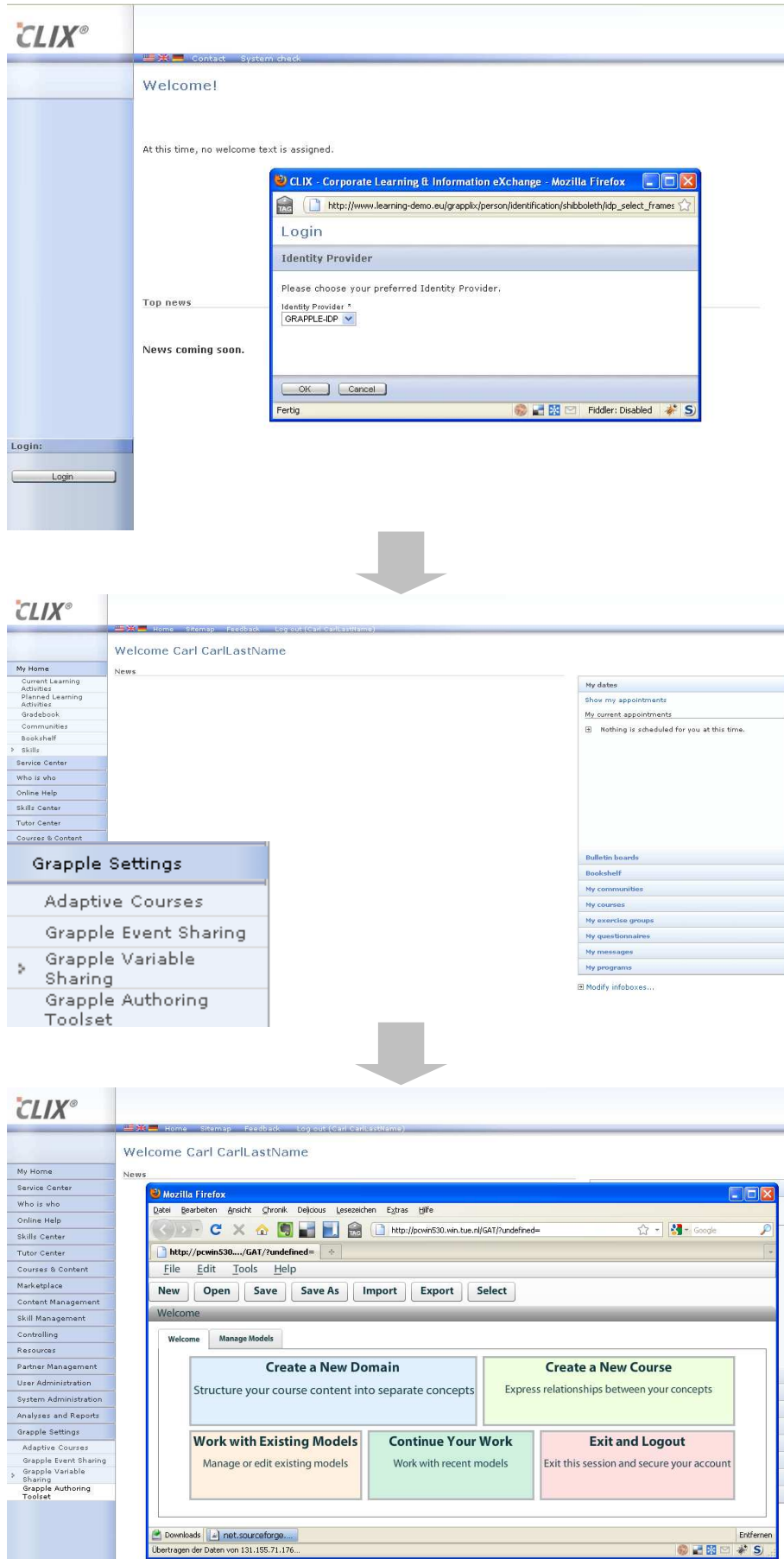
Figure 4: GRAPPLE-CLIX-prototype
