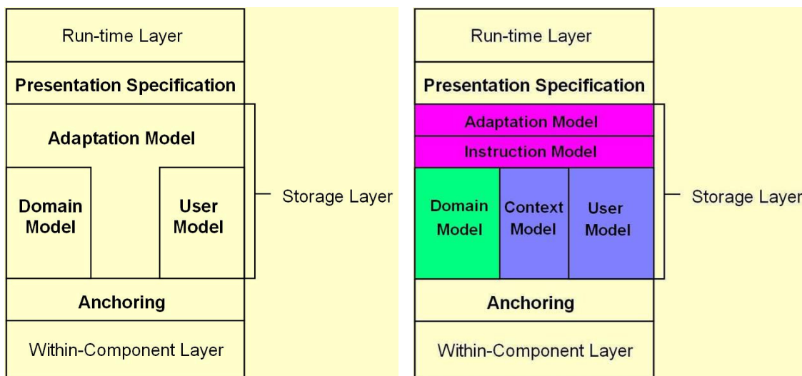
Figure 1: Adaptive Hypermedia Application Model (left) and its enhanced version (right)
